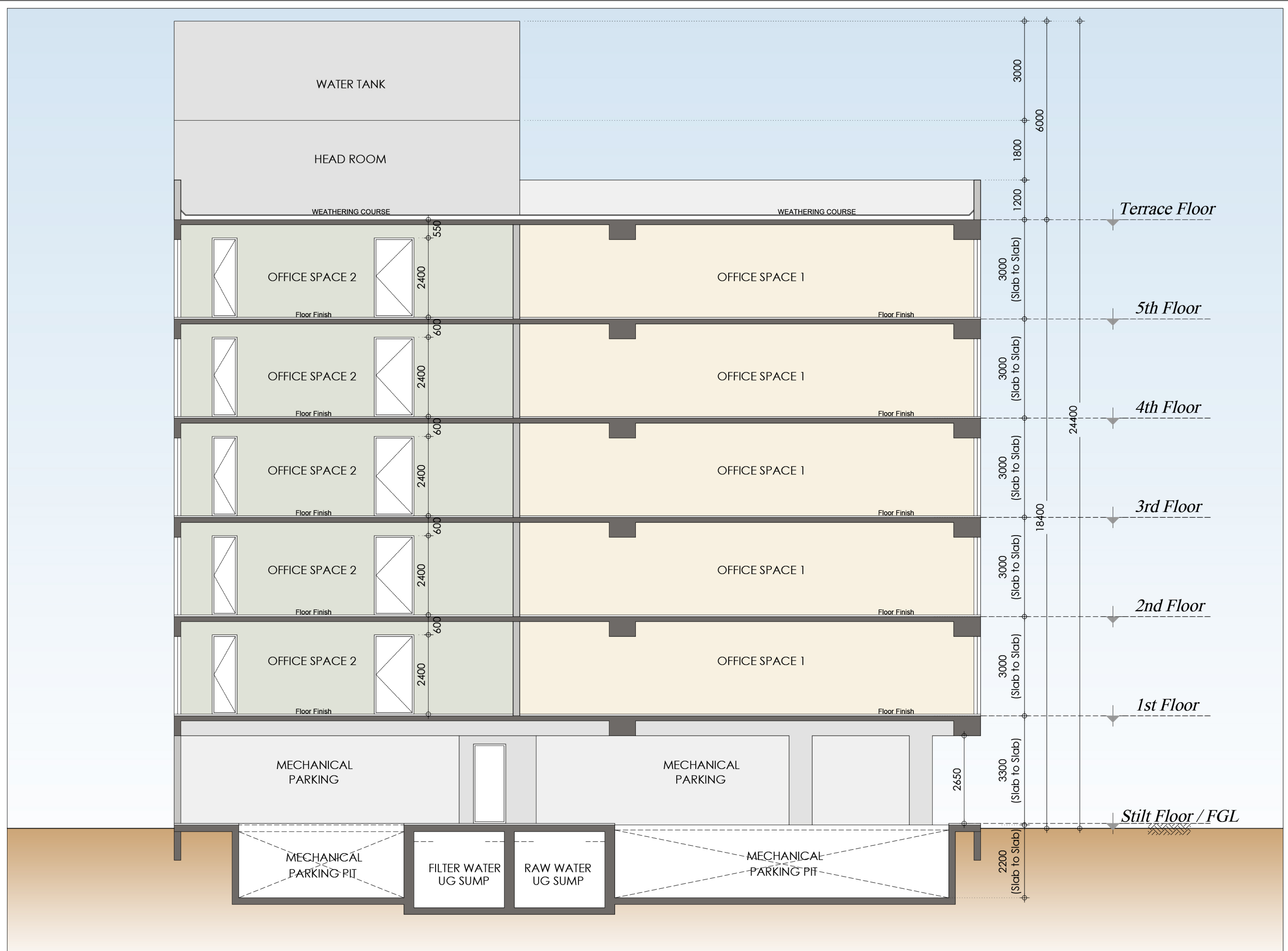
SCHEMATIC SECTION
